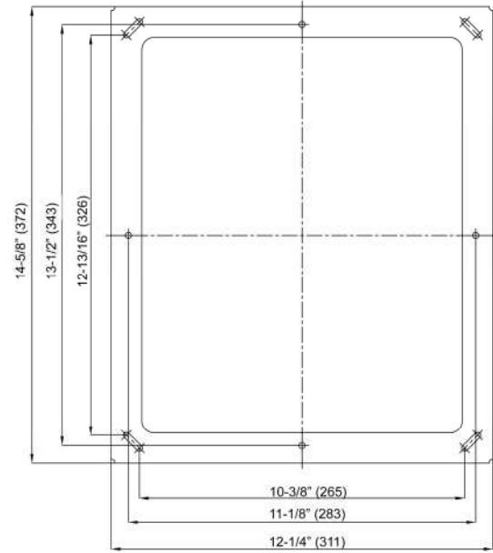
Mounting Template
