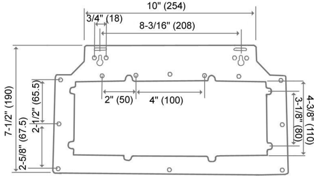
***Hood-Mounting Bracket
